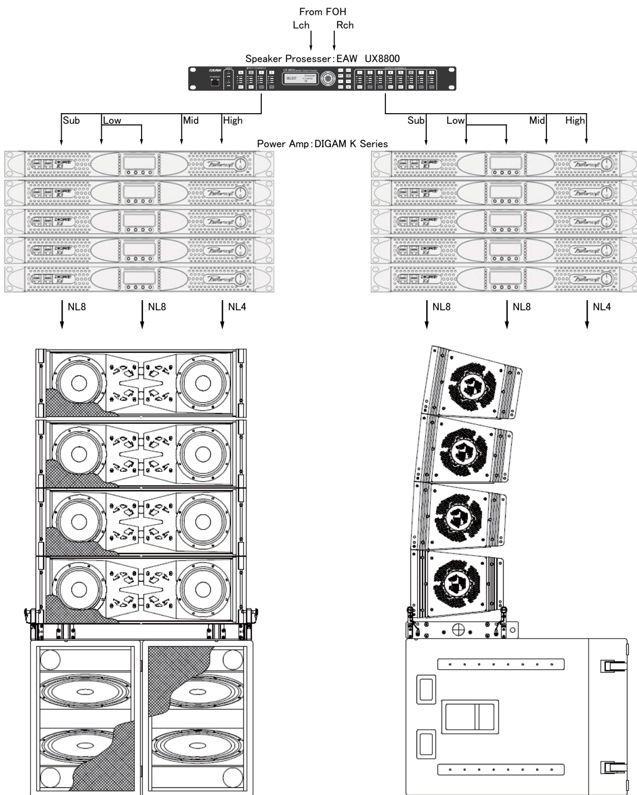
EAW KF740 + SB1002 4/2 System
